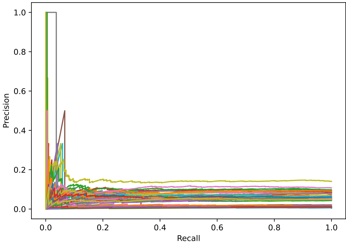
Precision-Recall Curves (Test)
