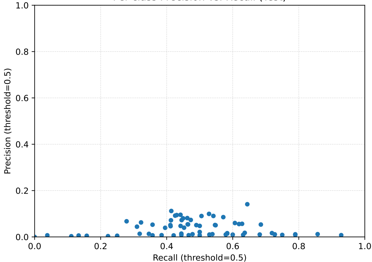
Per-class Precision vs. Recall (Test)
