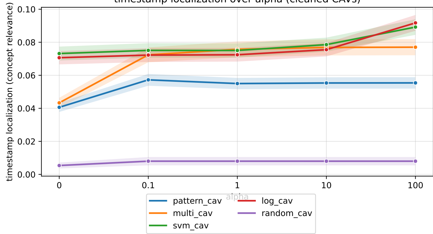
timestamp localization over alpha (cleaned CAVs)
