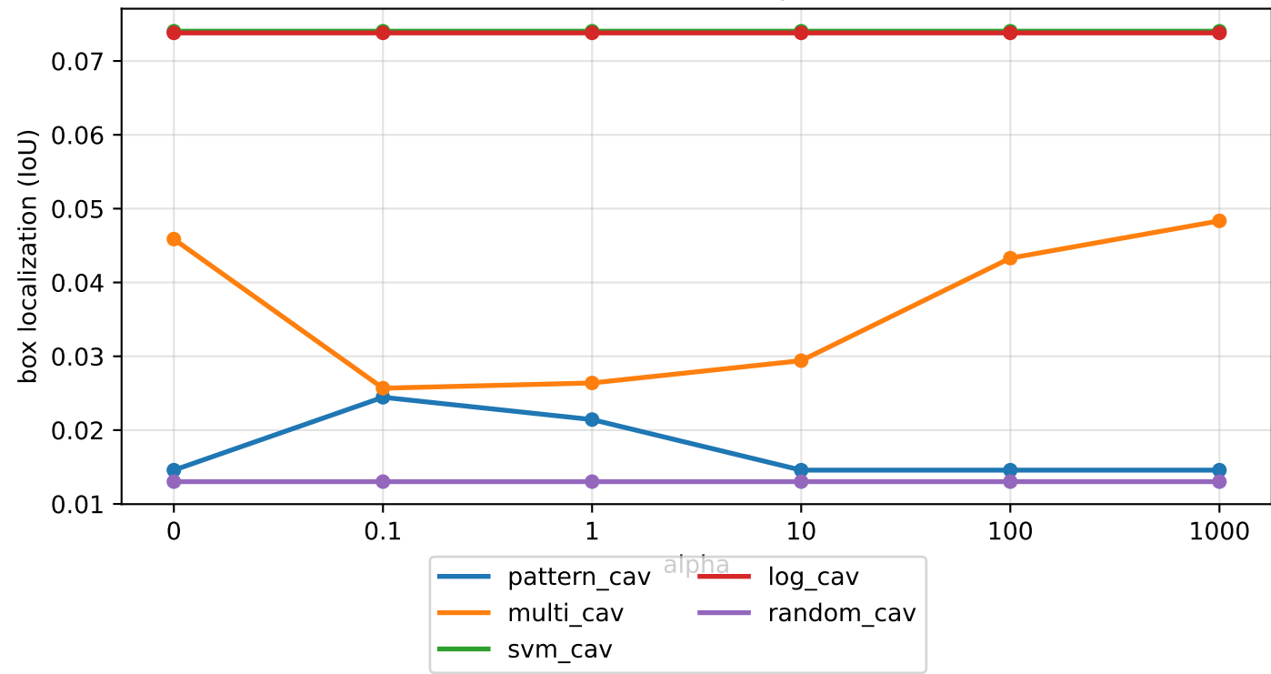
box IoU over alpha
