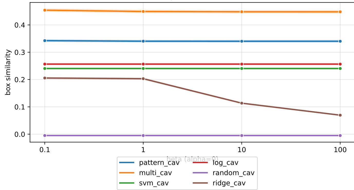
box alignment over beta
