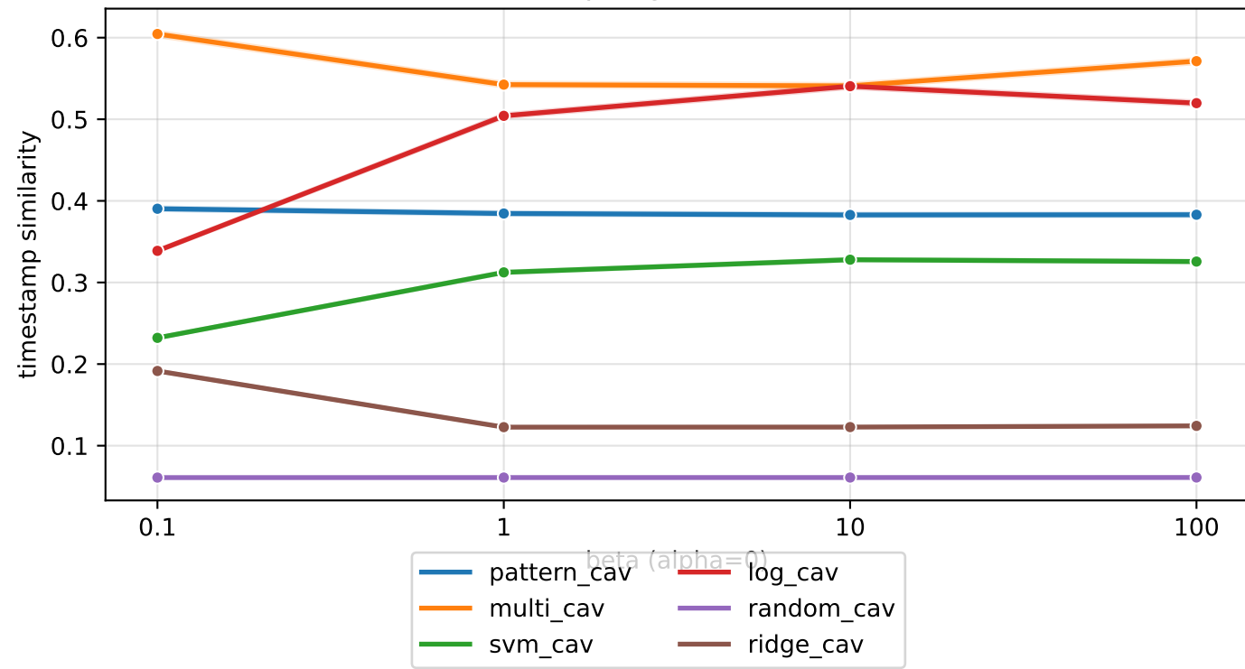
timestamp alignment over beta
