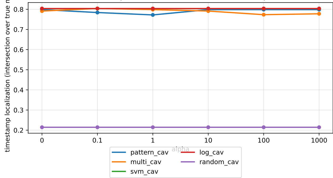
timestamp intersection over true mask over alpha
