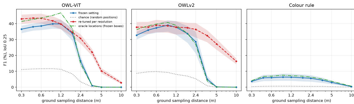
Figure 1. F1 against ground sampling distance at IoU 0.25 with area averaging, 400 held-out Paris and Khartoum chips. Solid blue: the setting frozen on development data, with its 95% interval. Dashed red: the setting re-tuned at each resolution. Dotted grey: chance (boxes moved to random positions). Dash-dot green: oracle locations (the frozen boxes moved onto random true building centres).
