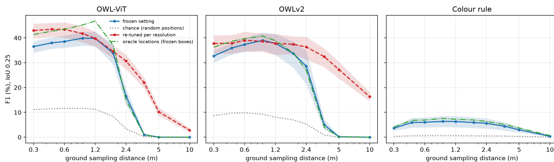
Figure 1. F1 against ground sampling distance at IoU 0.25 with area averaging, 400 held-out Paris and Khartoum chips. Solid blue: the setting frozen on development data, with its 95% interval. Dashed red: the setting re-tuned at each resolution. Dotted grey: chance (boxes moved to random positions). Dash-dot green: oracle locations (the frozen boxes moved onto random true building centres).
