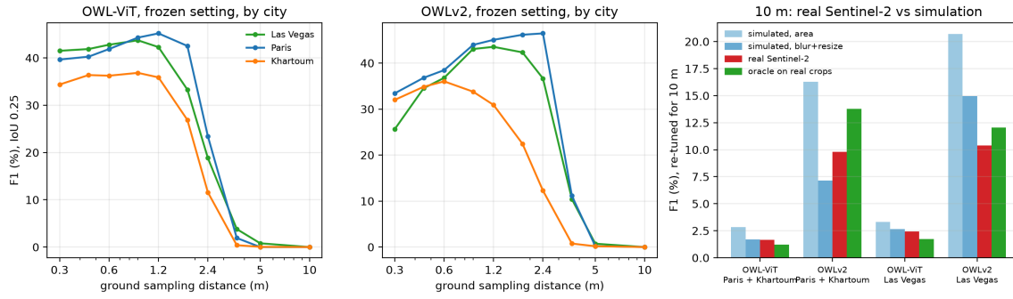
Figure 2. Left and middle: frozen-setting F1 against GSD in each city for OWL-ViT and OWLv2 (IoU 0.25, area averaging). Right: F1 at 10 m for the re-tuned settings on simulated 10 m images (two degradation methods), on real Sentinel-2 crops of the same footprints, and for the oracle-location baseline on the real crops.
