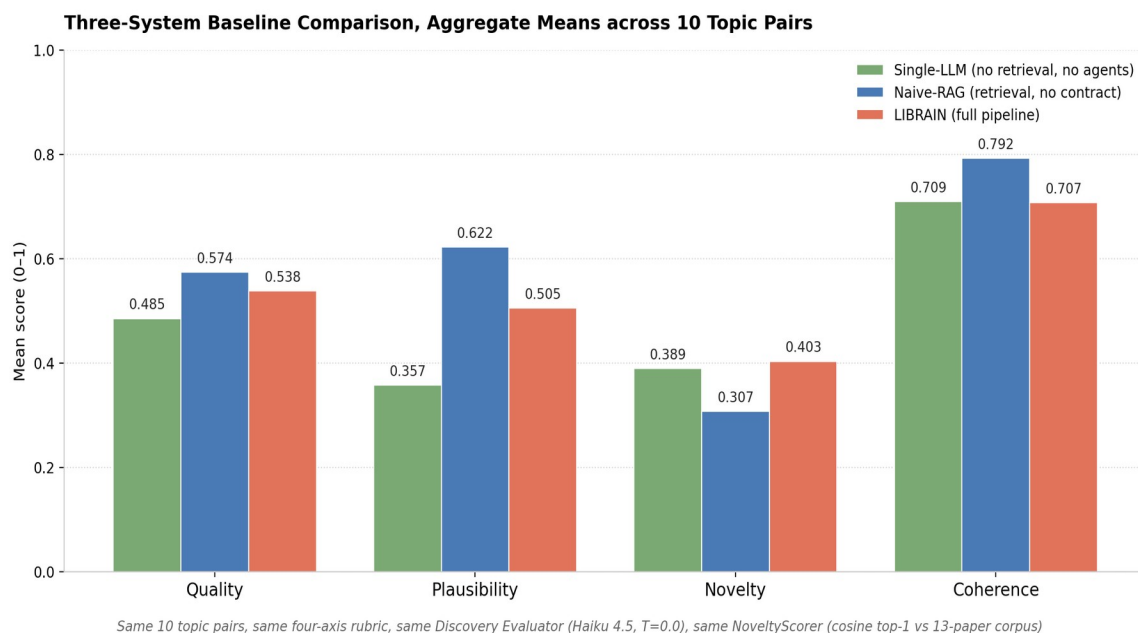
Figure 8. Aggregate-mean four-axis scores from the three-system baseline (ten topic pairs). Naive-RAG leads on plausibility and coherence, LIBRAIN leads on novelty by approximately 31 percent.
