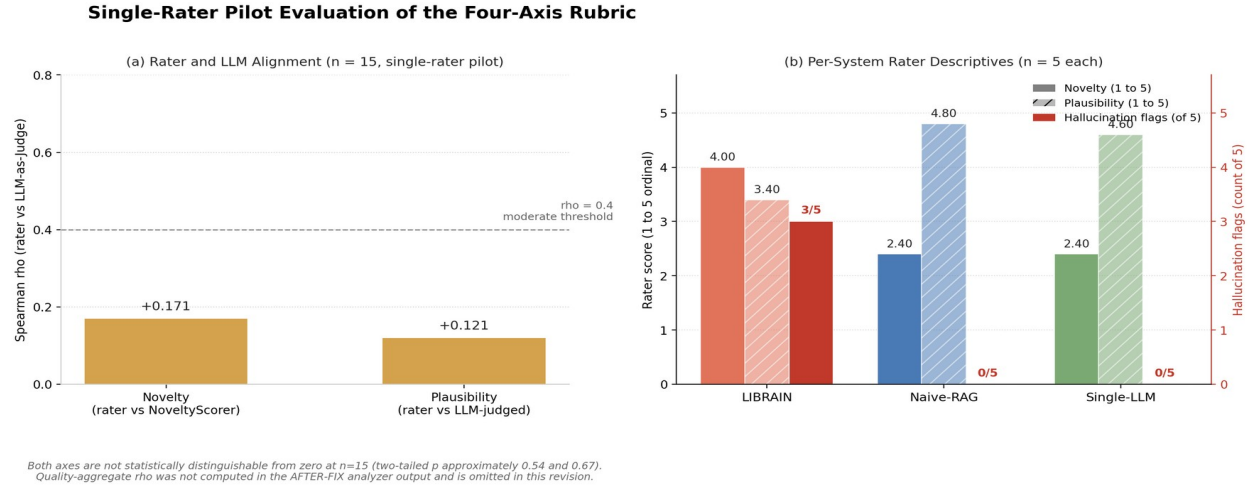
Figure 9. Single-rater pilot (n equals 15). (a) Per-axis Spearman rho: 0.17 for novelty, 0.12 for plausibility (not distinguishable from zero). (b) Per-system rater descriptives.
