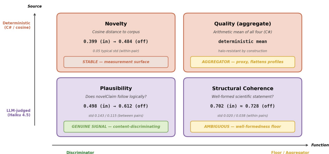
Figure 7. Four-axis sensitivity profiles. Plausibility discriminates content, structural coherence acts as a well-formedness floor.
