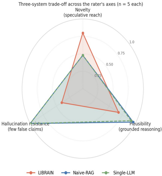
Figure 10. Novelty, plausibility, and hallucination trade-off across the three systems (a) and the claim-level contract added in Phase 3.A.5 (b).
