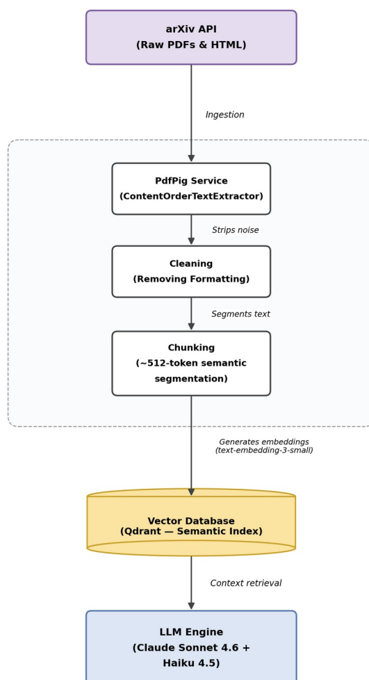
Figure 5. Data flow from arXiv source to the reasoning engine.
