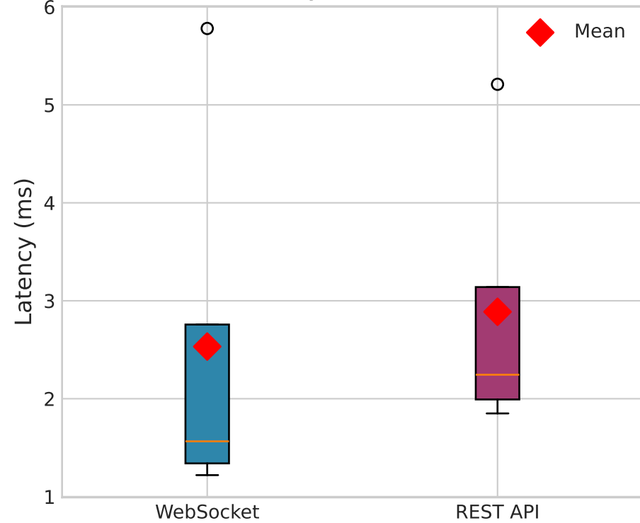
Latency Distribution
