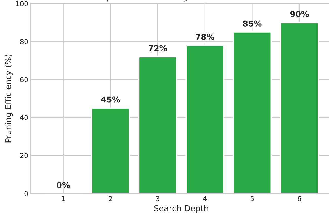
Alpha-Beta Pruning Node Reduction
