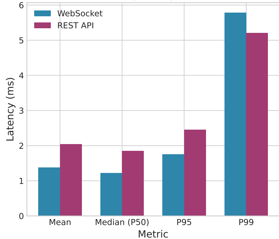
Latency Comparison
