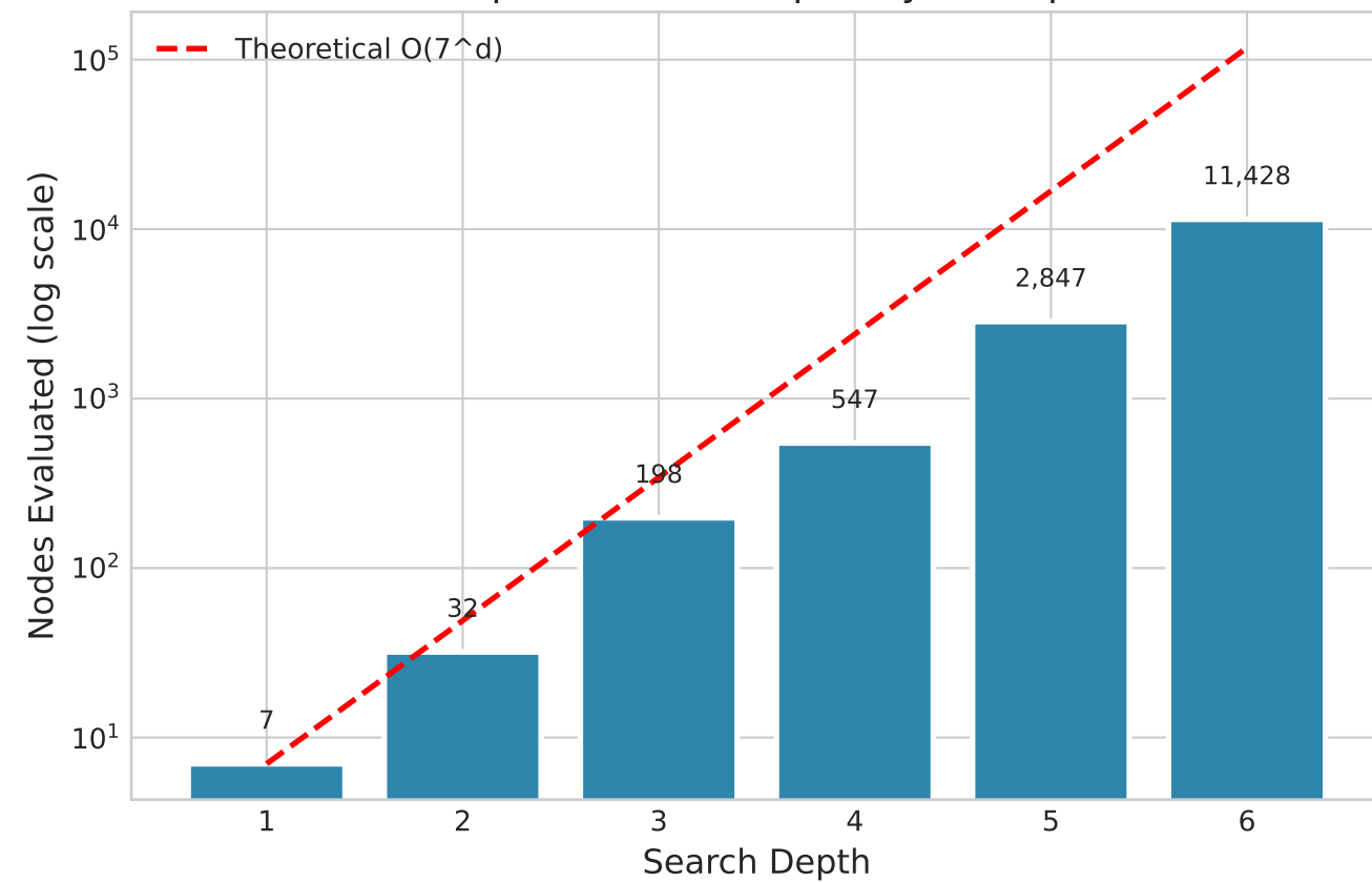
Computational Complexity Analysis
