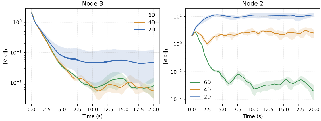
Figure 5: Comparison of L1 synchronization error under different observation configurations. Curves average three training-seed means, with ten common archived test initial conditions per seed; shading spans the minimum and maximum of the three seed means. This archived observation experiment uses fewer test initial conditions than the baseline and actuator-count comparisons.
