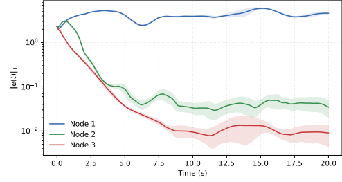
Figure 3: Synchronization error under different pinning nodes. Each curve averages three training-seed means, each evaluated on 20 common initial conditions; shading shows one sample standard deviation across the three seed means.
