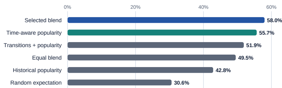
Fig. 2. Primary monthly macro Conditional Hit Rate@2. Popularity is a substantive comparator.
