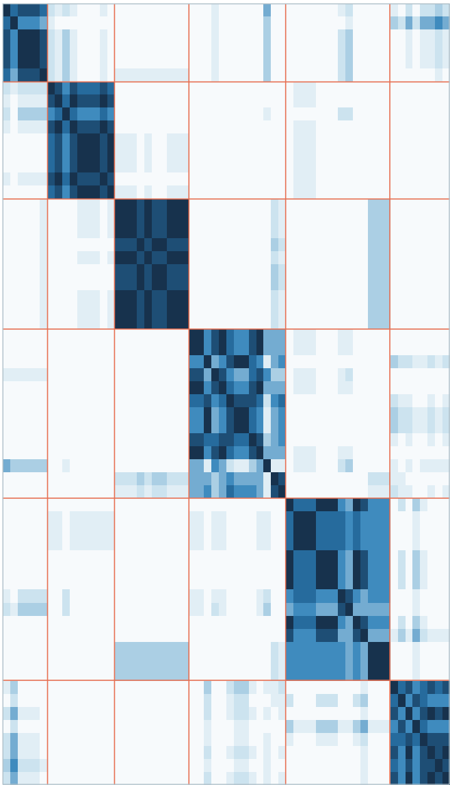
Patient-patient co-assignment
