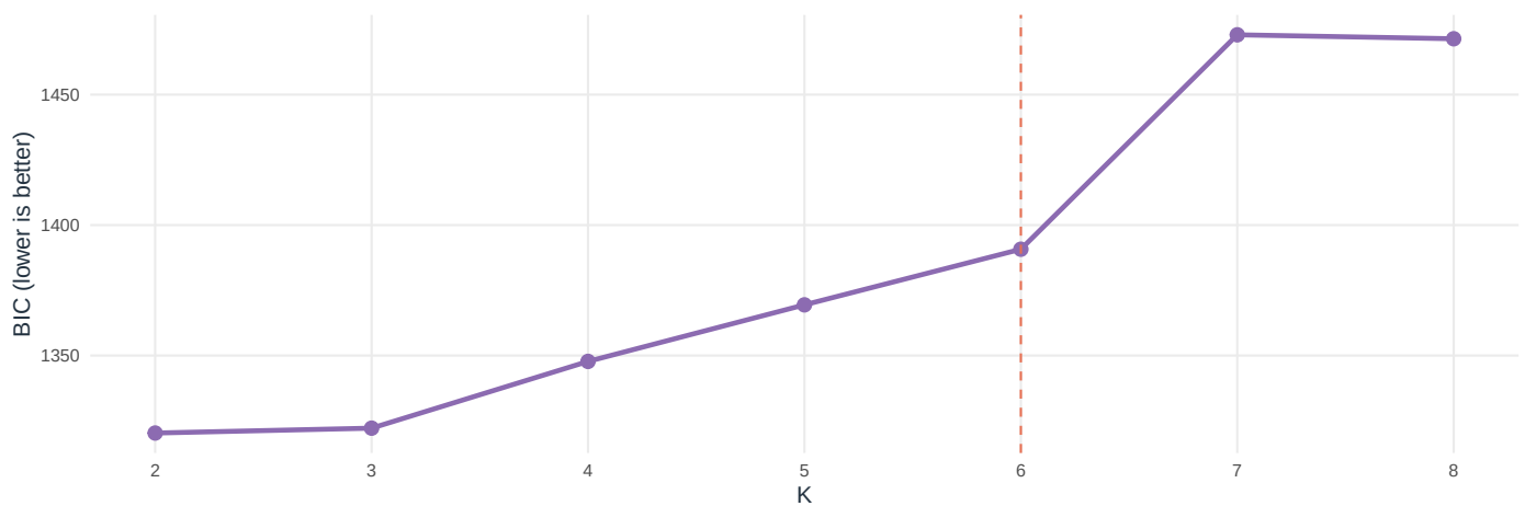
Latent mixture
