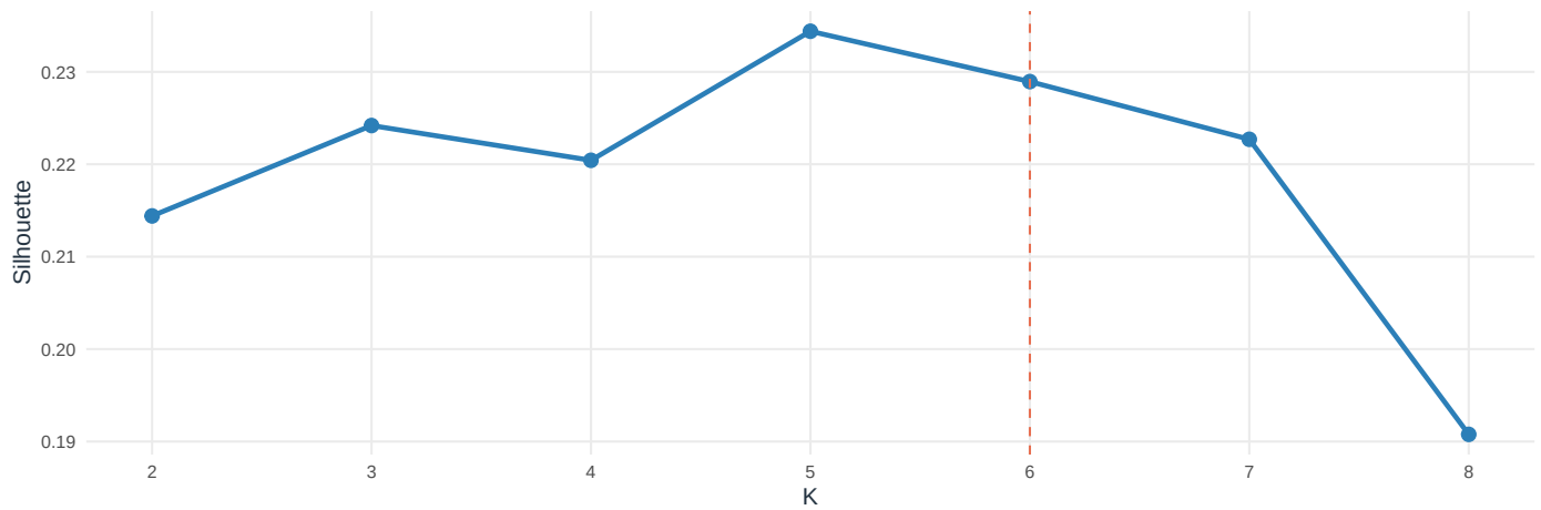
Gower + PAM
