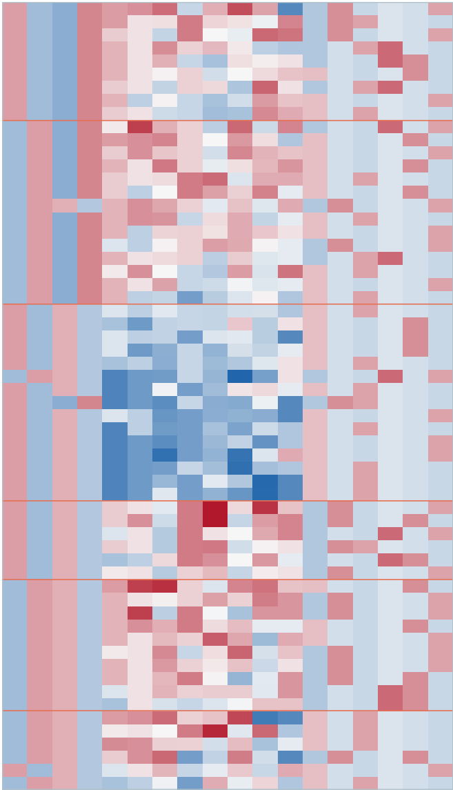
Patient-feature heatmap (18 encoded columns)
