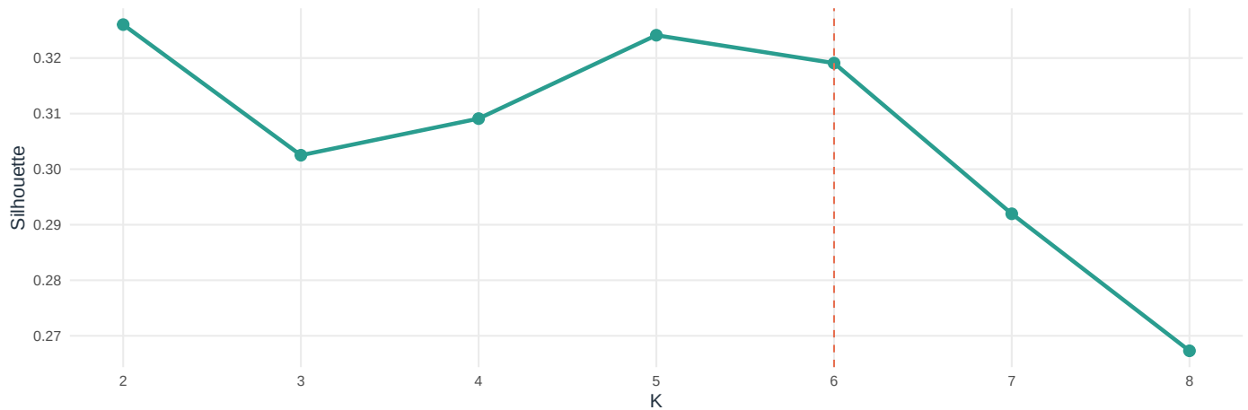
FAMD-style + k-means
