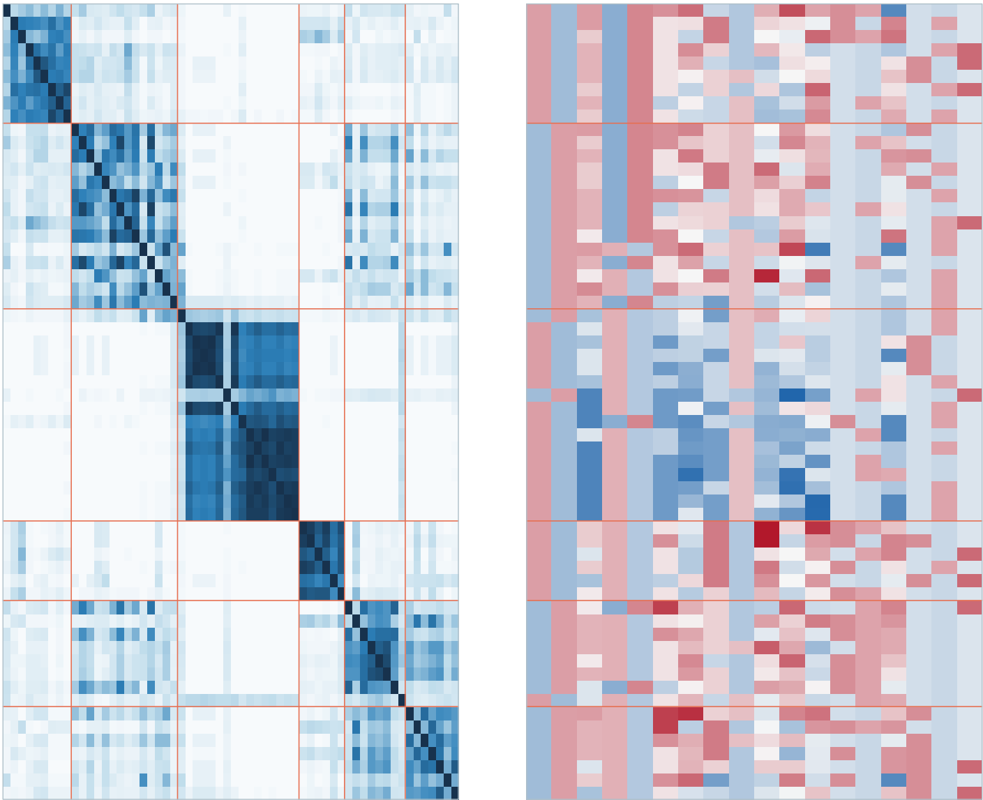
Patient-patient co-assignment
