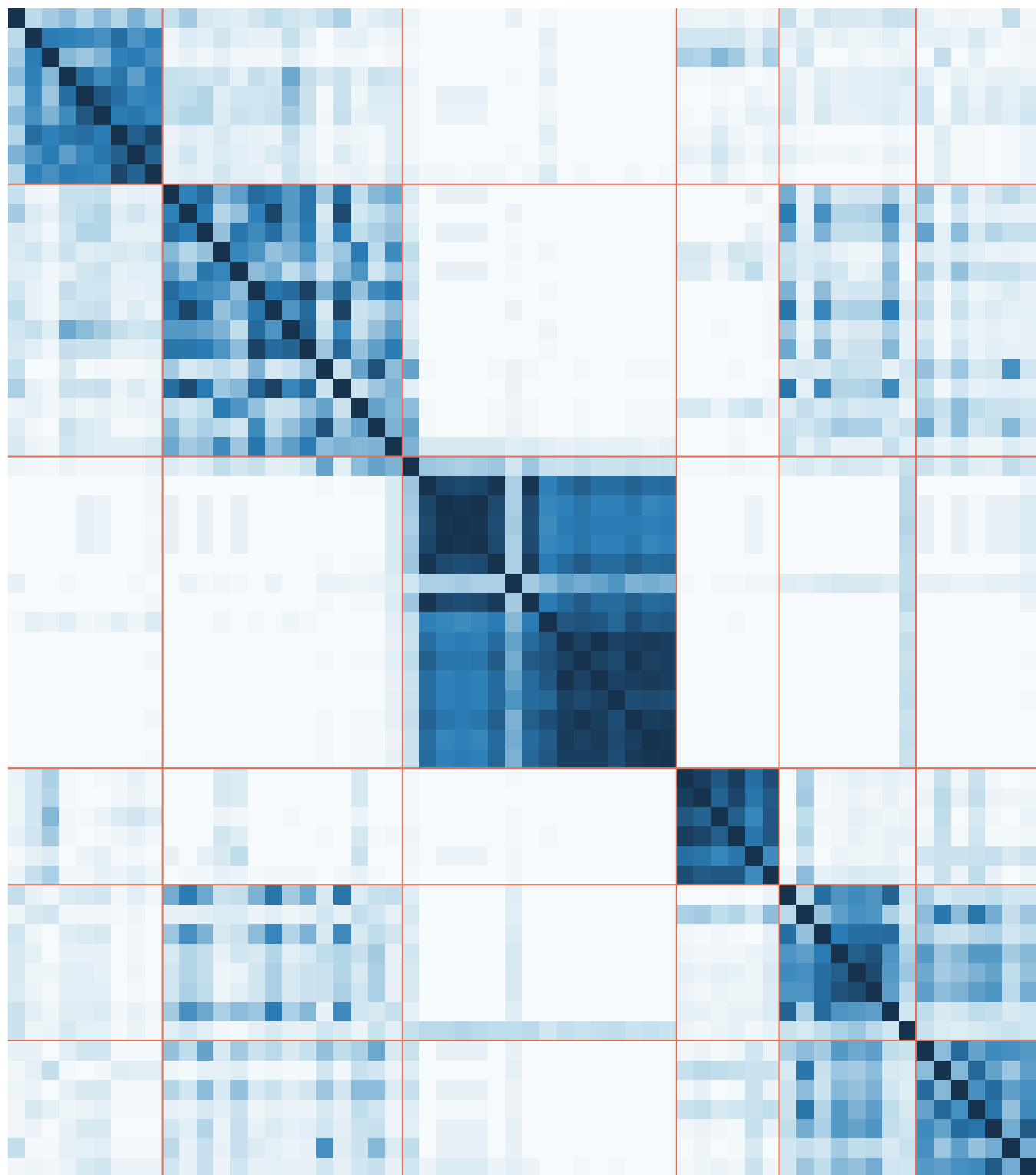
Patients sorted by consensus cluster, then latent axis 1
