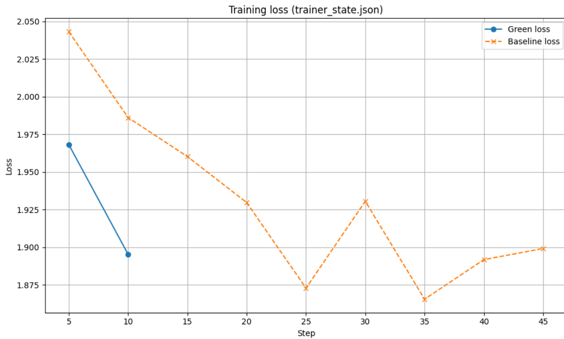
Figure 4: Loss curve
