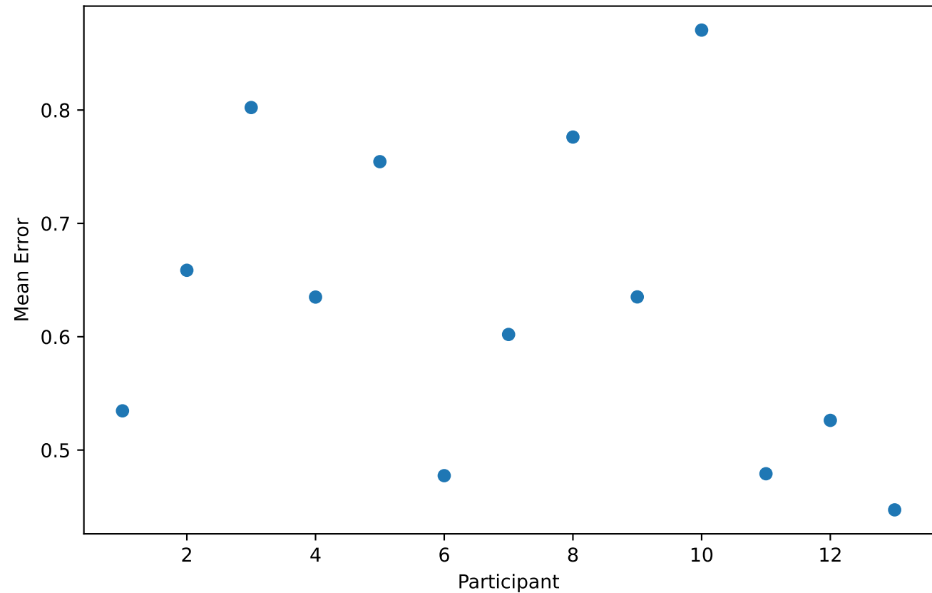
Participant Influence Diagnostics
