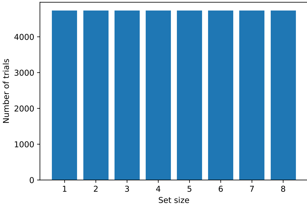
Set Size Distribution
