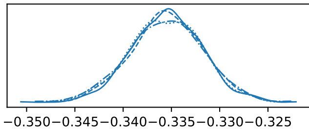
beta
