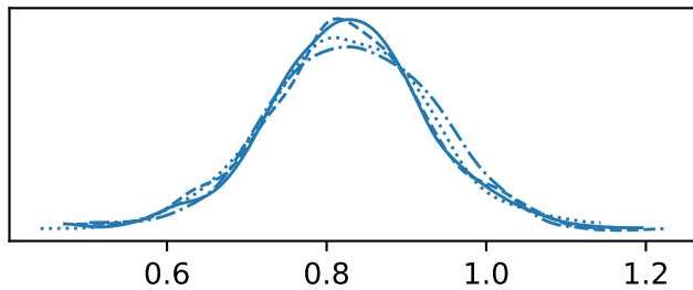
alpha
