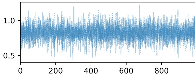
alpha
