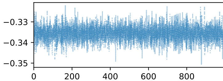
beta
