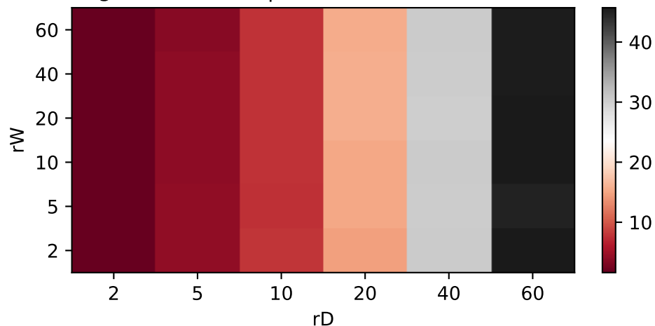
Avg eff-rank(dW) | W0 low-rank, dW high-rank
