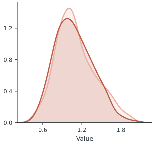
Band half-width
