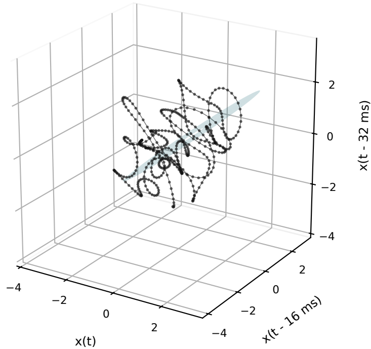
1-torus: planar band
