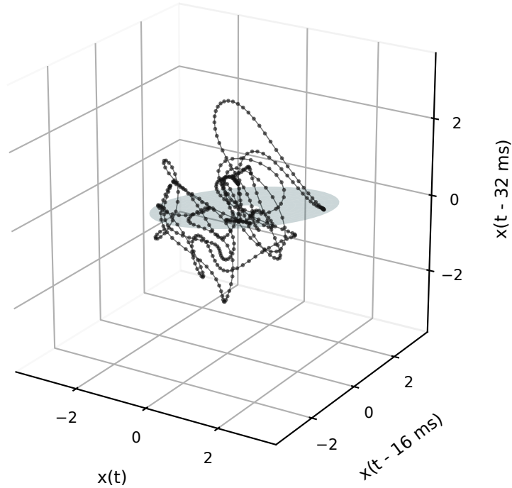
1-torus: planar band
