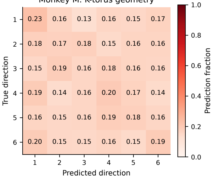
Monkey M: K-torus geometry
