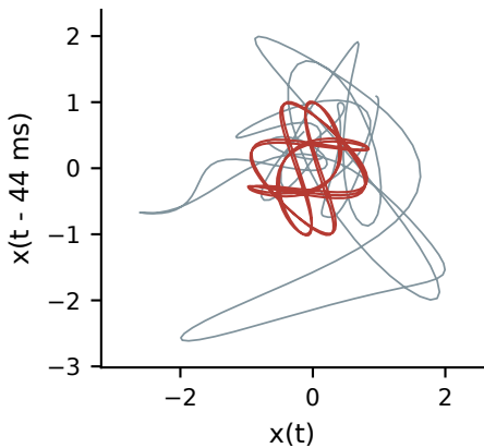
Monkey M: K=2 , m=5 , delay=44 ms Display only; full-coordinate fit
