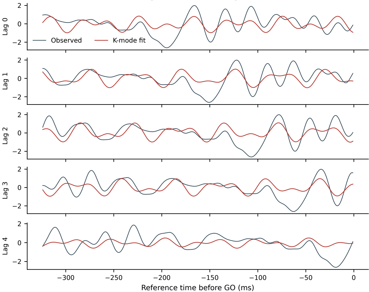
Monkey M: K=2, m=5, delay=44 ms
