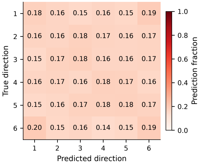
Monkey M: Torus features
