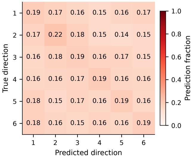
Monkey T: Torus features
