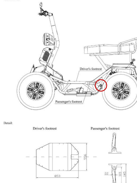
Variant DS: driver + passenger footrests (2)
