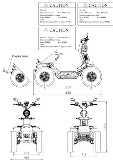
Variant SS dimension drawing
