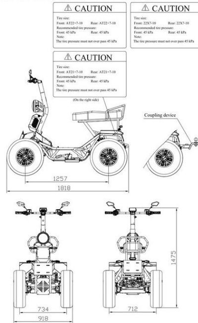
Variant DS dimension drawing (height 1475 mm)
