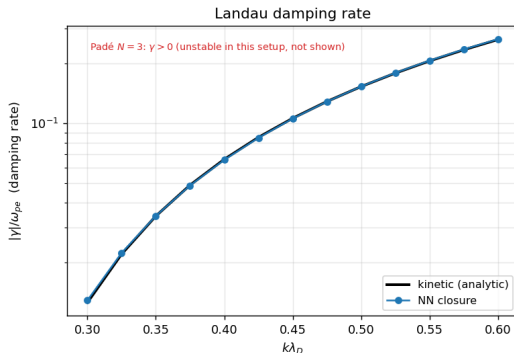
Landau damping on a single warm Maxwellian (same NN as BoT, no retraining)
