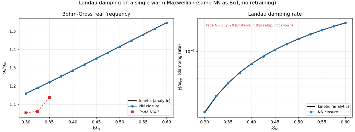
Figure 16: Landau damping of Langmuir waves on a single warm Maxwellian, using the same NN checkpoint trained for BoT. Left : Bohm-Gross real frequency. Right : damping rate, log scale. The NN closure reproduces the kinetic ground truth (textbook values: \gamma/\omega_{pe} = -0.0126 at k\lambda_D = 0.3 , -0.1534 at k\lambda_D = 0.5 , etc.) to better than 1% across the range. Padé N = 3 in this setup gives the wrong frequency and is unstable ( \gamma > 0 ); not shown on the log-damping axis. See text.
