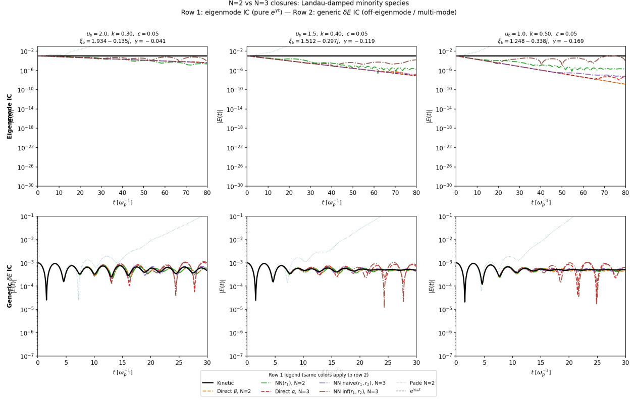
Figure 18: Top row: eigenmode-projected IC. Direct- \beta N=2 and direct- \alpha N=3 (exact on eigenmode) decay cleanly along the reference slope e^{\gamma_{\text{kin}} t} . Both NNs also decay but level off at later times as approximation error accumulates. The kinetic N_v=96 curve is nearly flat: O(10^{-14}) mixing with van Kampen quasi-continuum modes dominates after \sim 10 e-folds. Bottom row: generic \delta E IC; kinetic (black) is ground truth.
