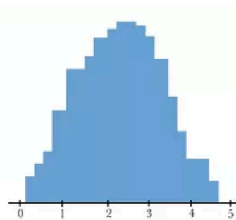
symmetric, unimodal
