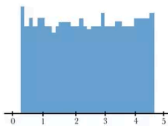
uniform
