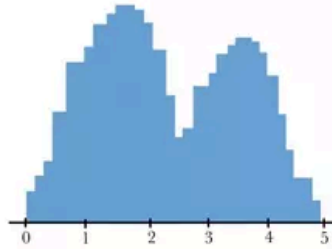
bimodal
