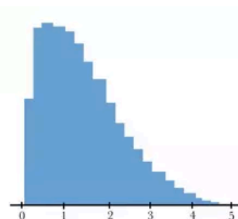
skew right
