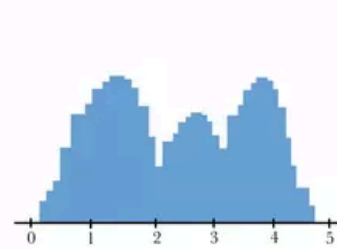
multimodal
