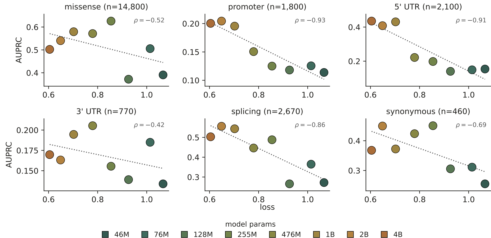
Parameter scaling — loss vs VEP AUPRC by variant type
