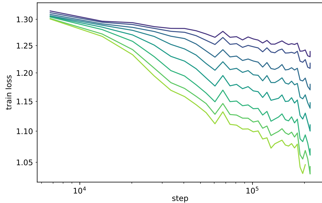
Parameter scaling — loss curves & scaling law N = 46\text{M} - 4\text{B} , D = 84\text{B} , C = 2.5 \times 10^{19} - 1.2 \times 10^{21}
