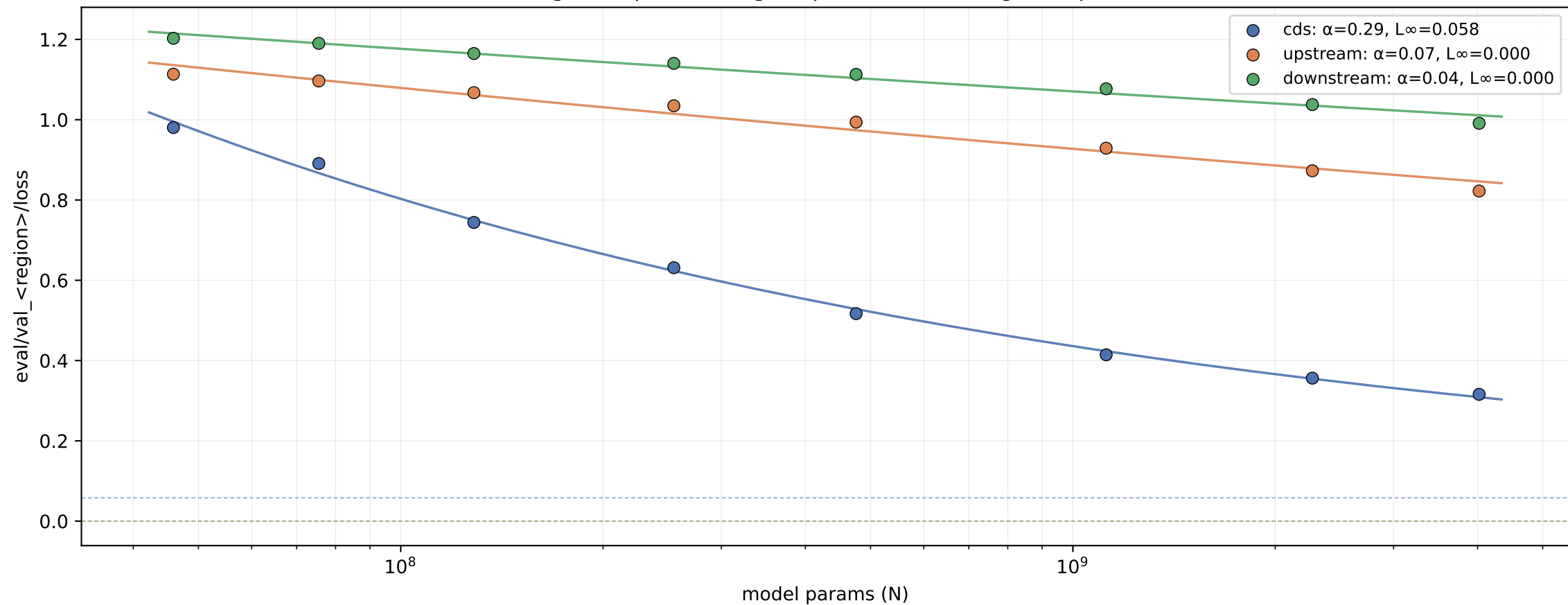
Per-region Kaplan scaling fit (parameter scaling sweep, v0.5)
