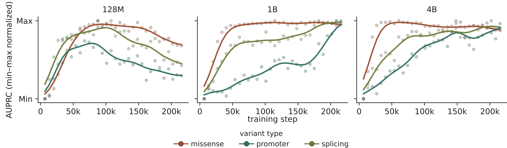
Parameter scaling — VEP AUPRC across training steps
