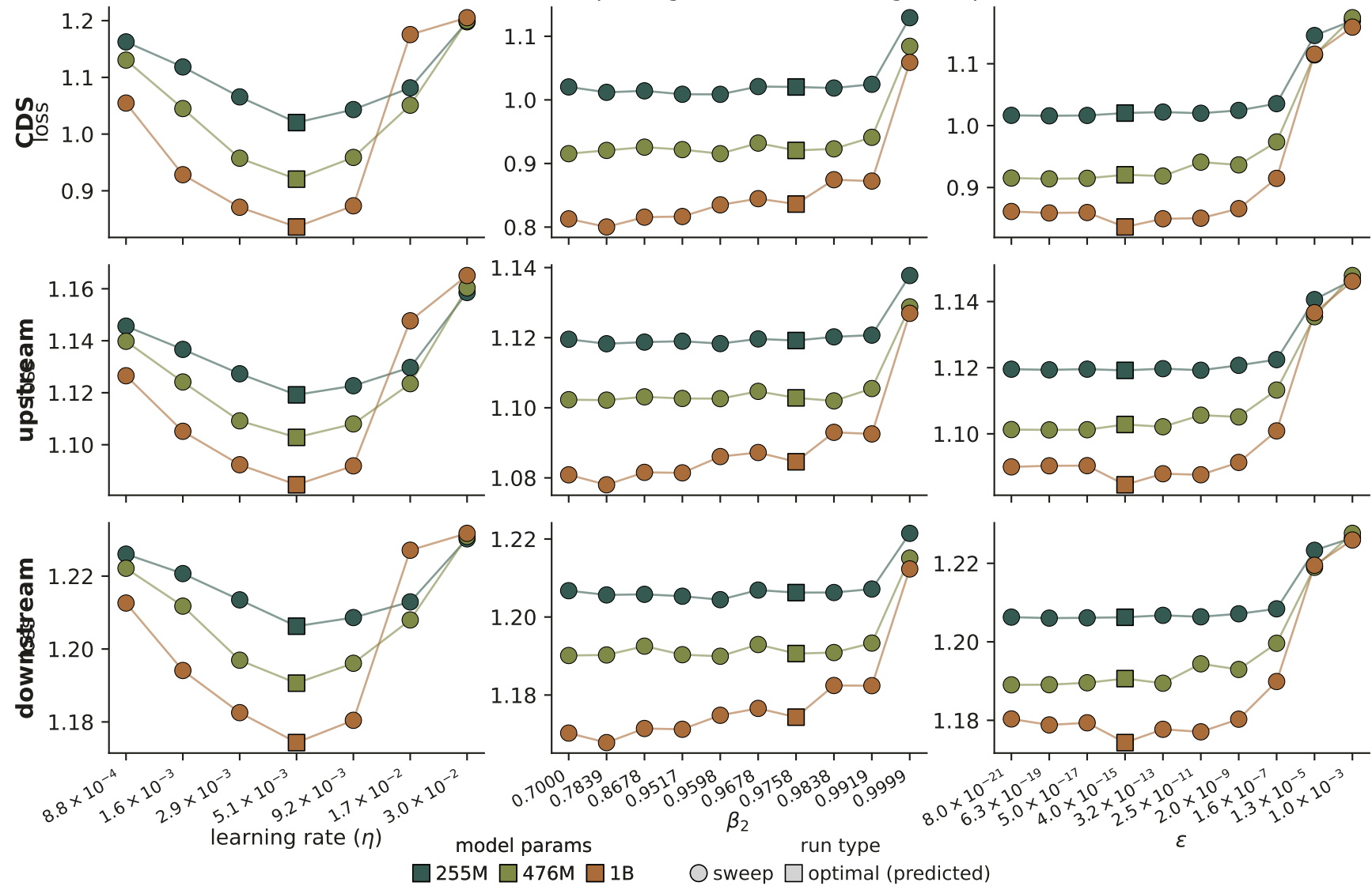
Transfer validation — per-region loss vs learning rate, \beta_2 , and \varepsilon
