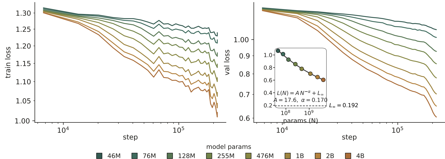
Parameter scaling — loss curves & scaling law N = 46\text{M} - 4\text{B} , D = 84\text{B} , C = 2.5 \times 10^{19} - 2.1 \times 10^{21}
