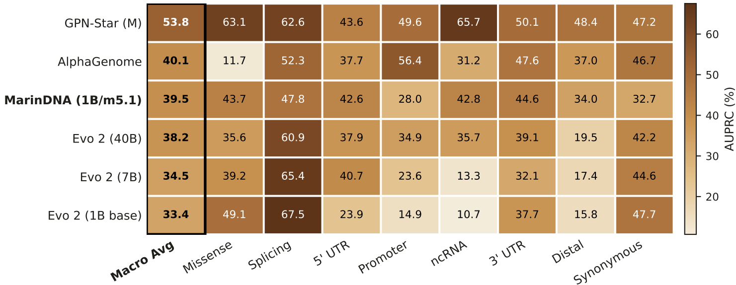
Mendelian VEP benchmark — AUPRC (%)
