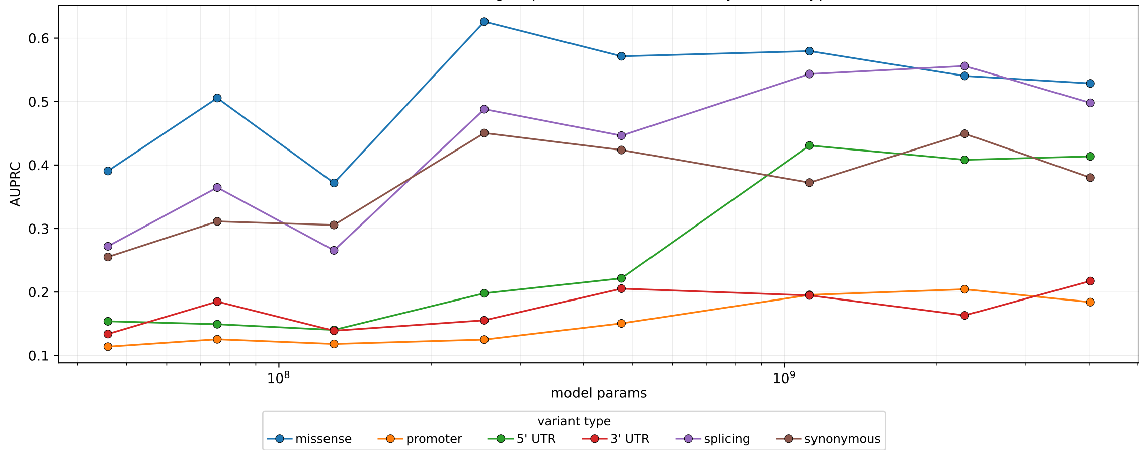
Parameter scaling — params vs VEP AUPRC by variant type
