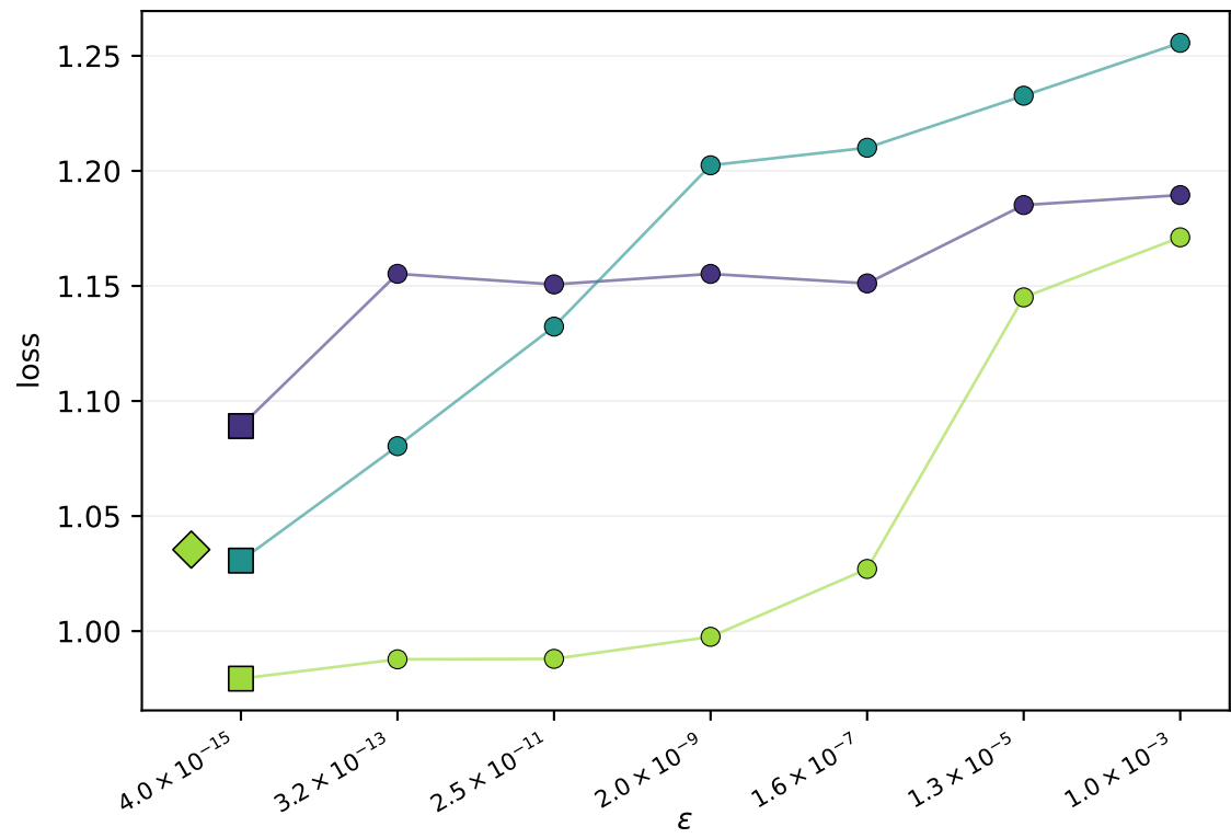
Transfer validation — loss vs \beta_2 and \varepsilon
