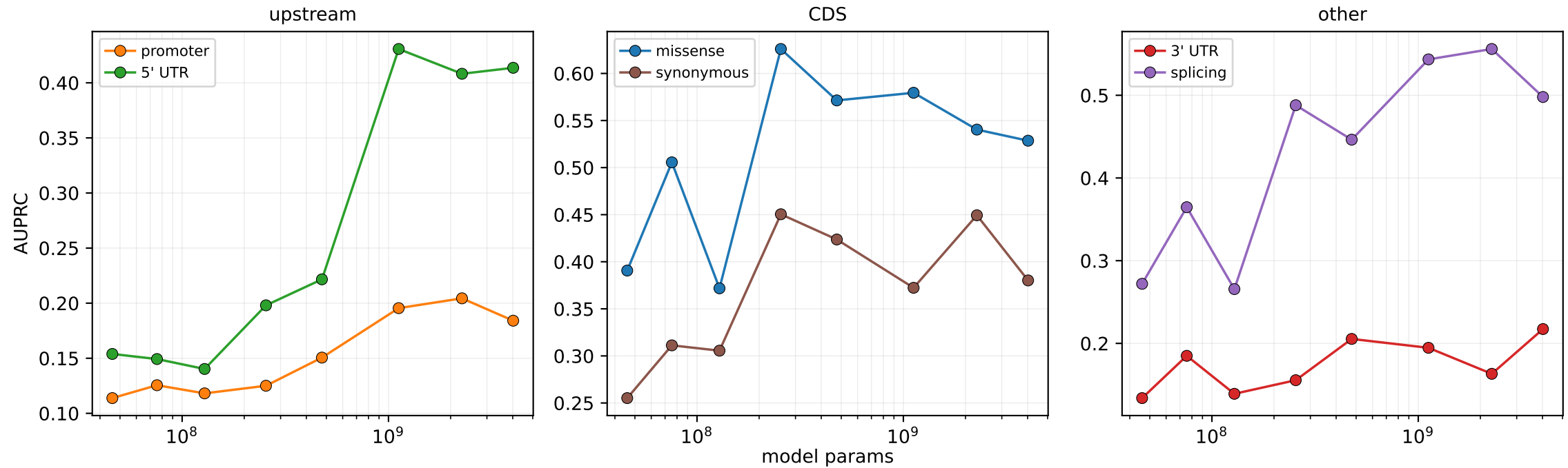
Parameter scaling — params vs VEP AUPRC by variant type
