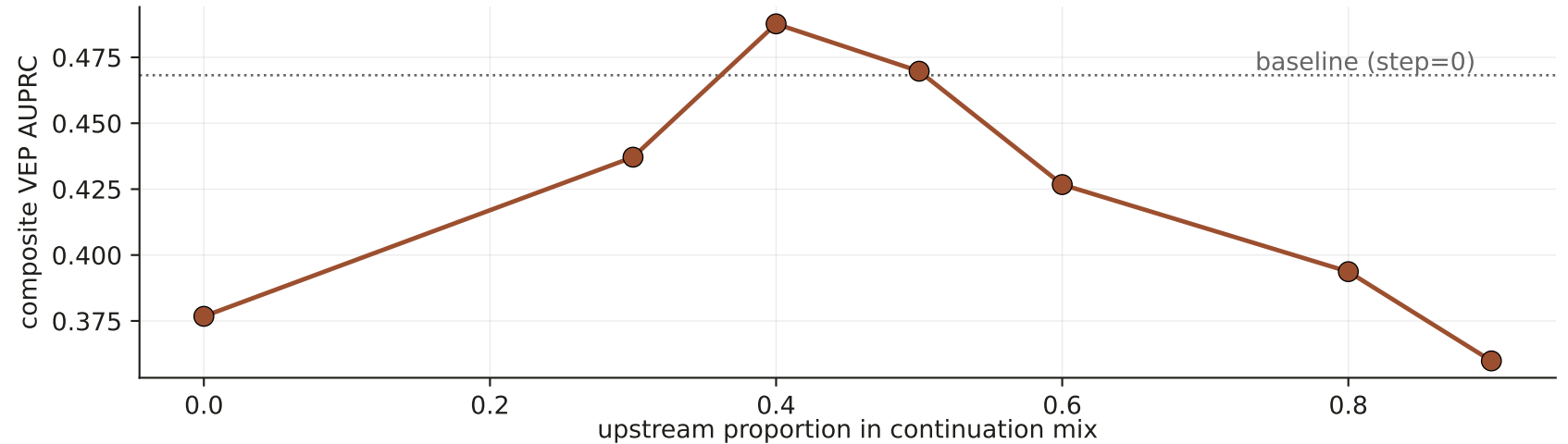
Continued pretraining from uniform mixture
