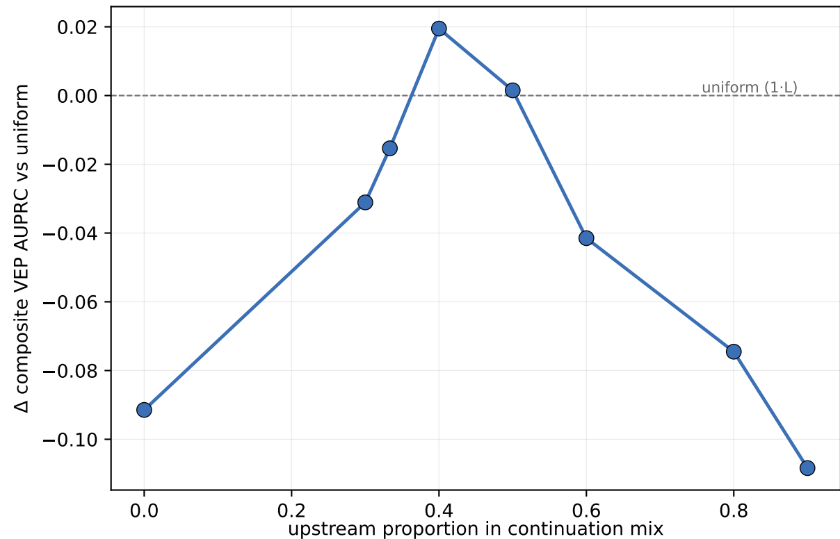
Continued pretraining from uniform — VEP AUPRC vs upstream proportion
