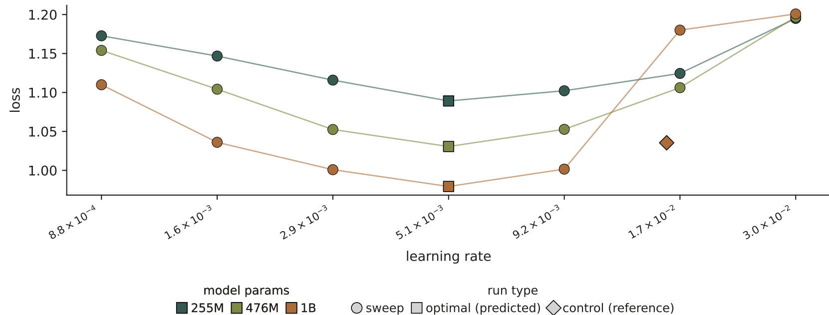
Transfer validation — loss vs learning rate N = 25\text{M}, D = 2.5\text{B}, C = 4 \times 10^{17} \rightarrow N = 255\text{M} - 1\text{B}, D = 10\text{B}, C = 1.6 - 6.8 \times 10^{19}
