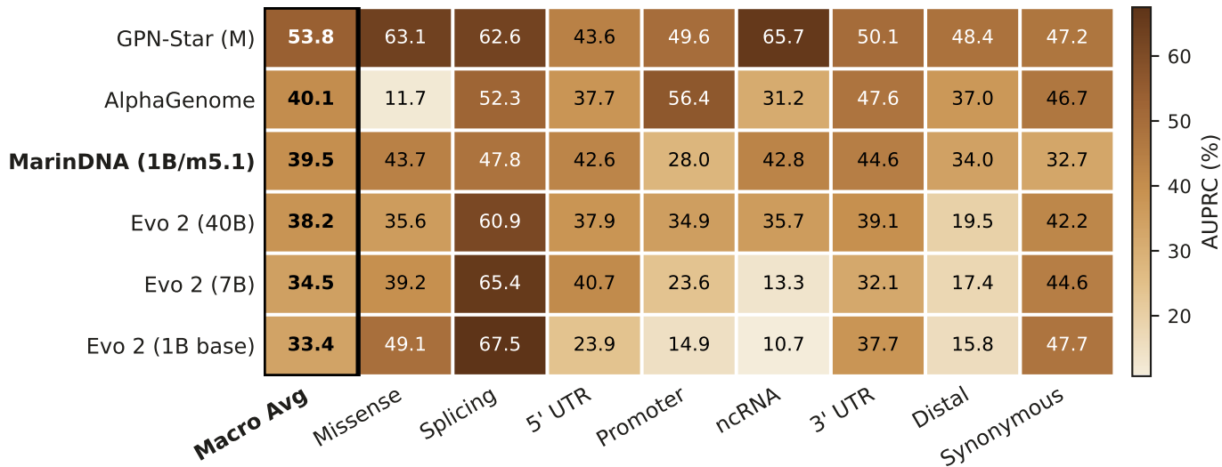
Mendelian VEP benchmark — AUPRC (%)
