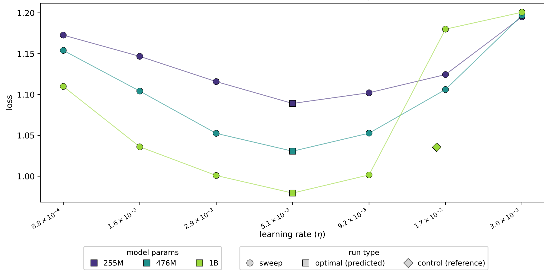
Transfer validation — loss vs learning rate
