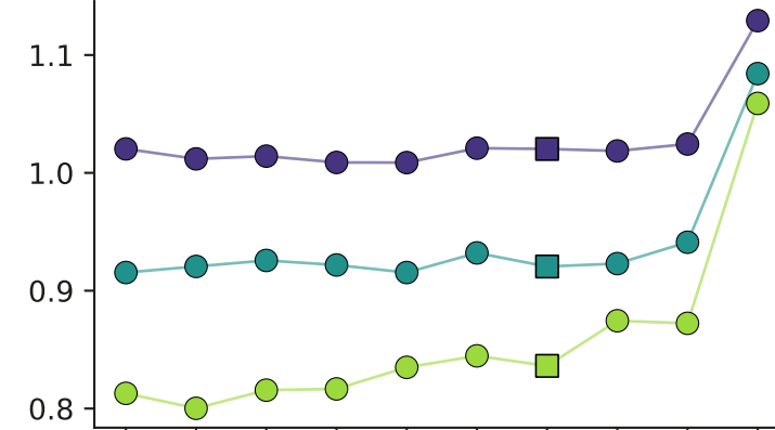
Transfer validation — per-region loss vs learning rate, \beta_2 , and \varepsilon
