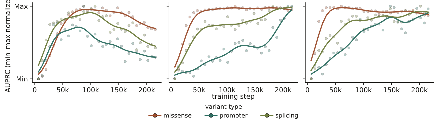
Parameter scaling — VEP AUPRC across training steps
