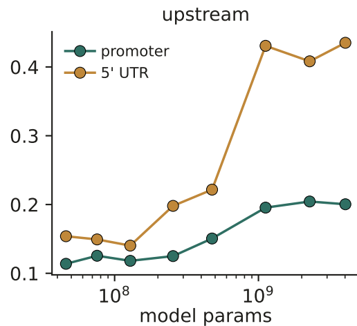
Parameter scaling — params vs VEP AUPRC by variant type
