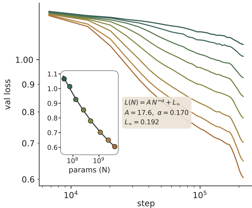
Parameter scaling — loss curves & scaling law N = 46\text{M} - 4\text{B} , D = 84\text{B} , C = 2.5 \times 10^{19} - 2.1 \times 10^{21}
